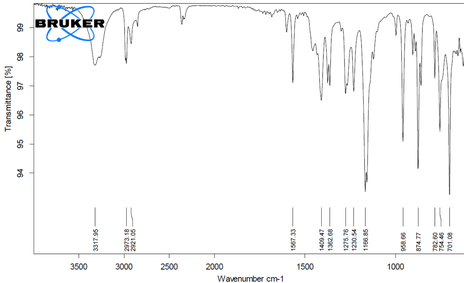
IR of 1-bromo-3,5-bis(1-hydroxy-1-methylethyl)benzene ( 2 )
